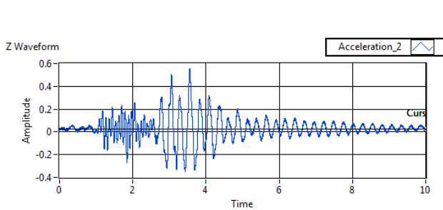
Fig. 11 Vertical acceleration Z - time representation ( v_0 = 10\text{km/h} with traction)
